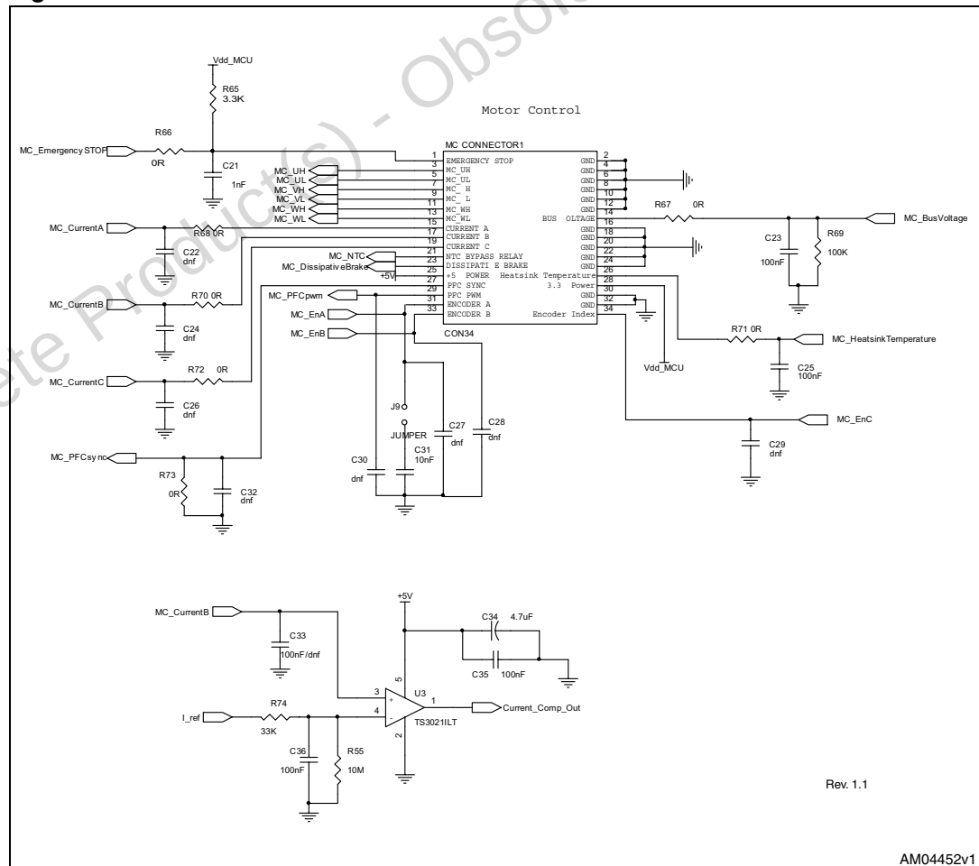
Figure 4. MC connector
